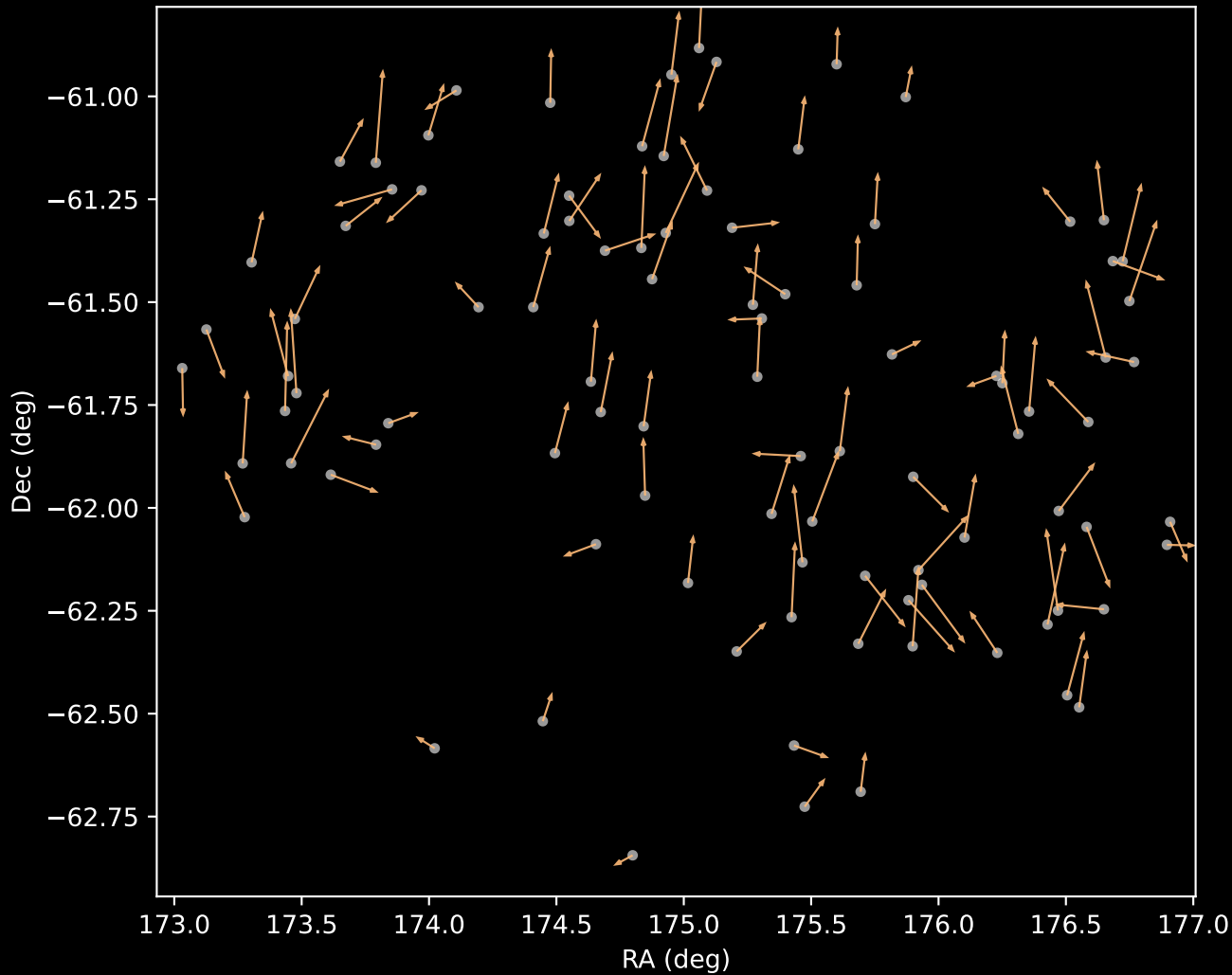
GALAH DR4 Cluster 3 Proper Motion Vectors (n=97)
