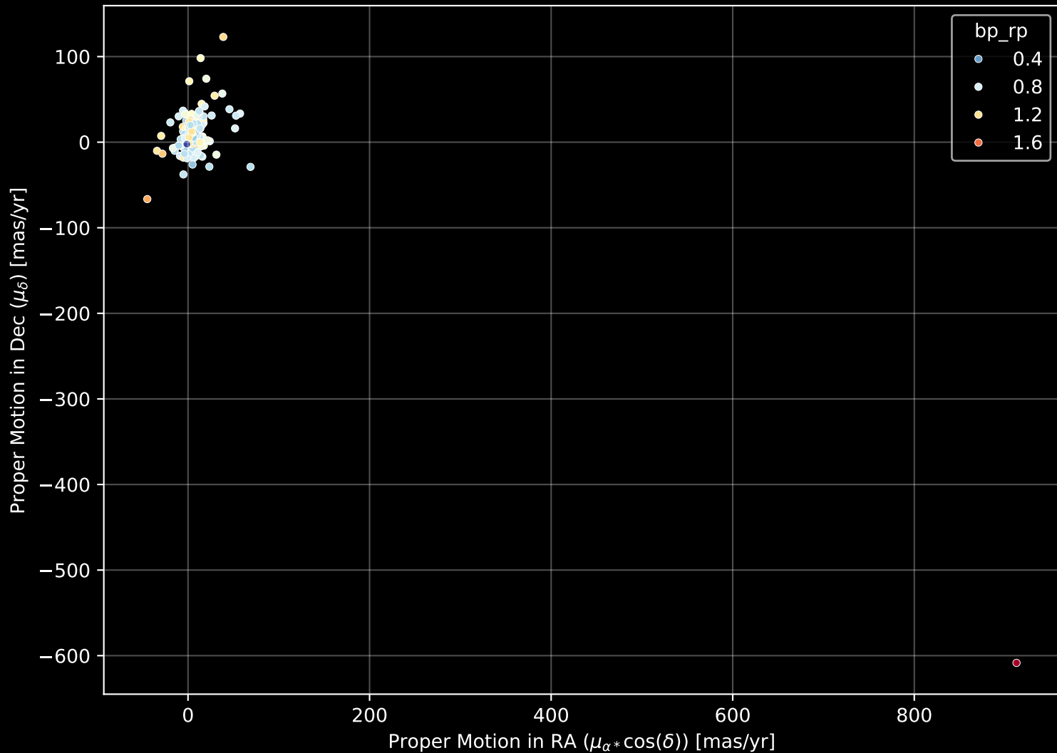
GALAH DR4 Field: [7156] Proper Motion Diagram (n= 182)
