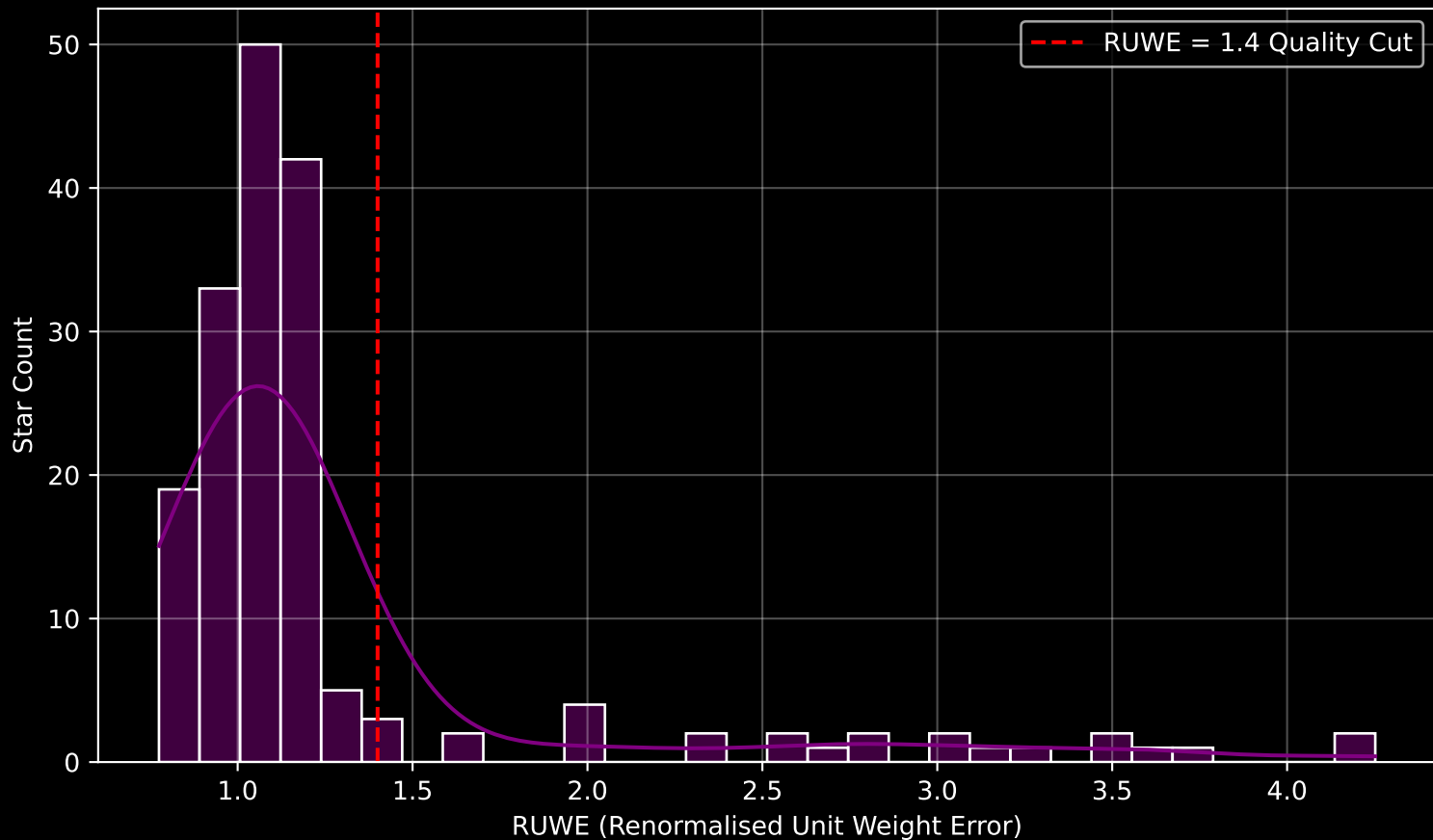
GALAH DR4 Field [7156] RUWE Distribution (n= 175)
