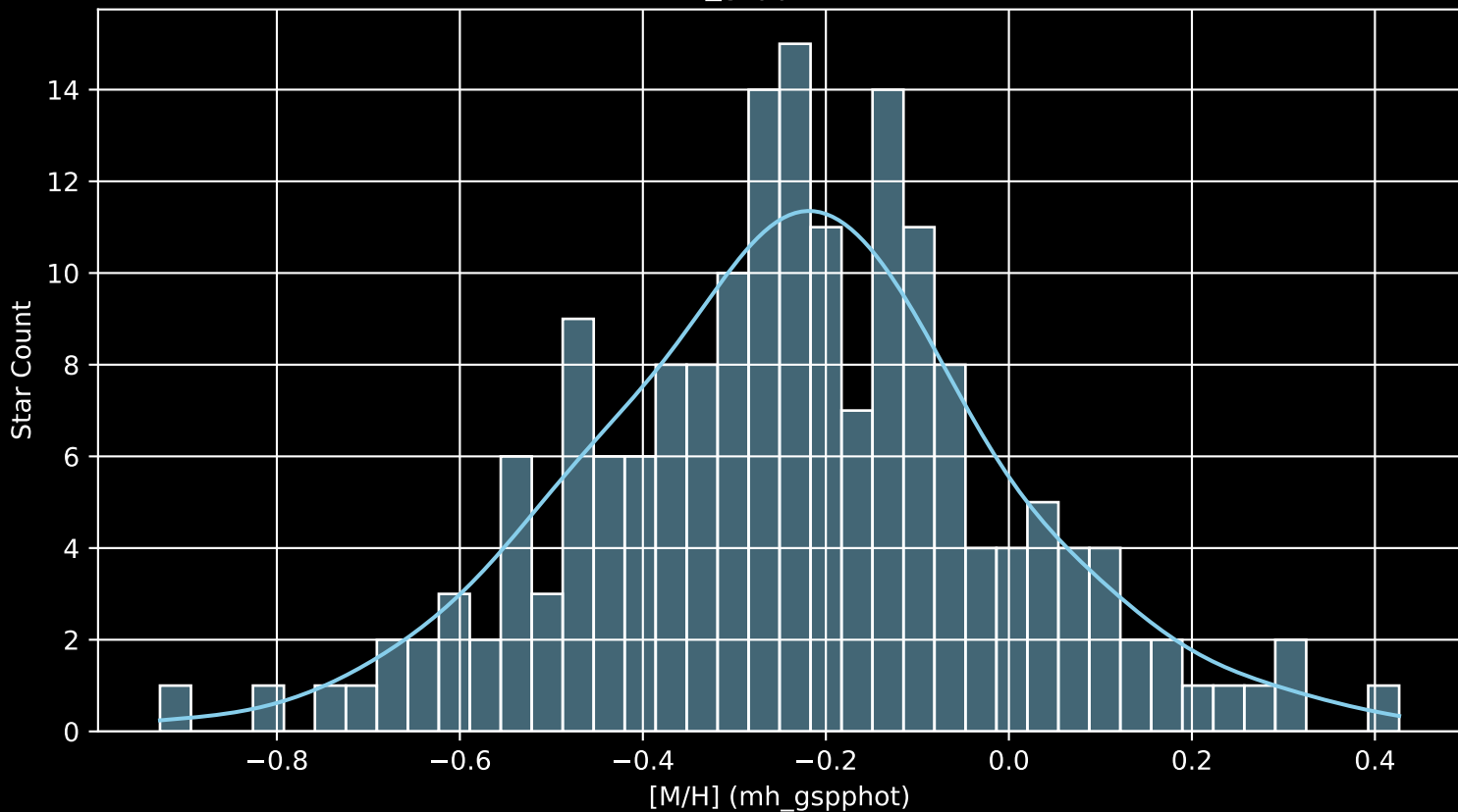
GALAH DR4 Field: [7156] [M/H] (mh_gspphot) (n= 180)
