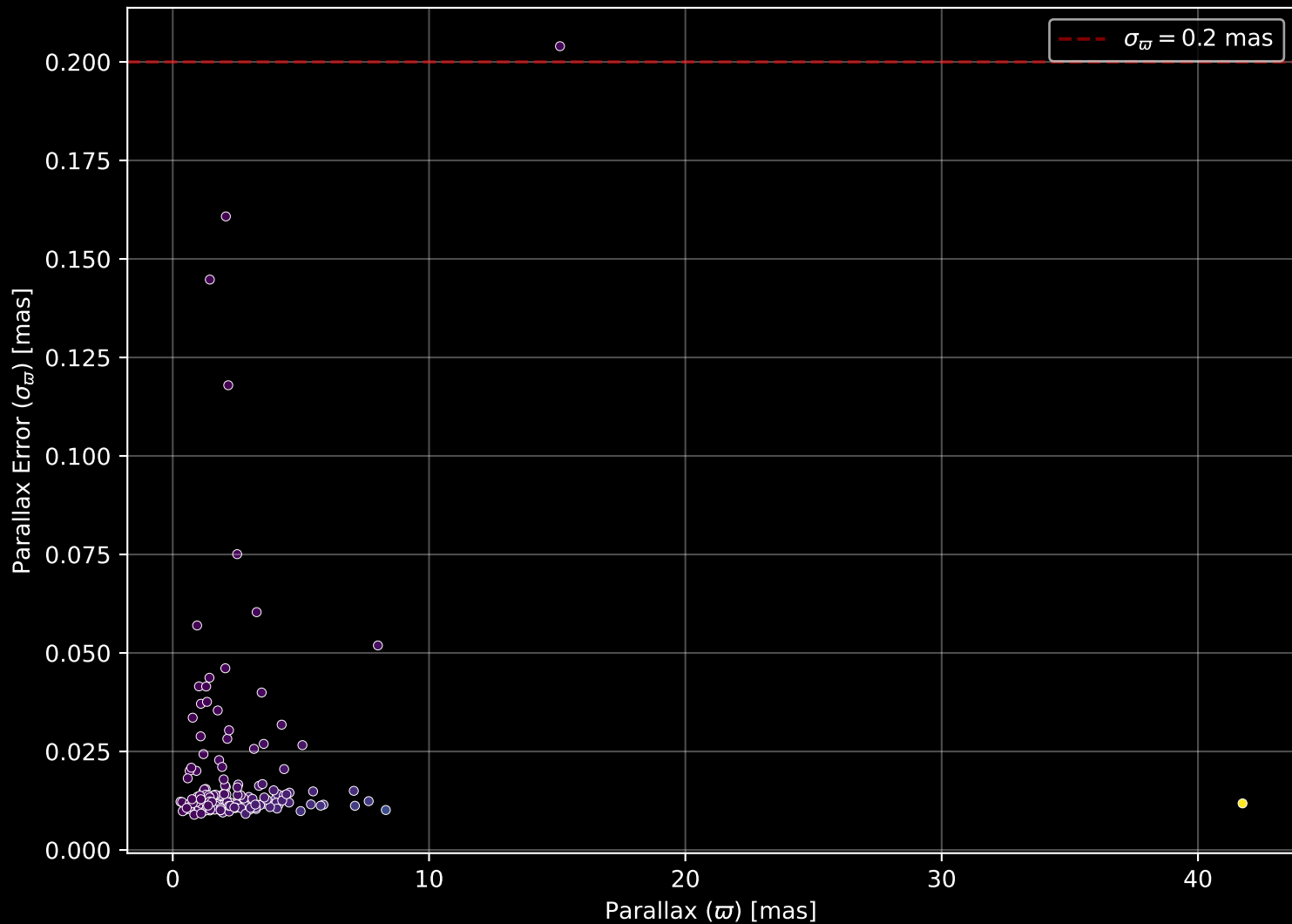
GALAH DR4 Field: [7156] Parallax Quality (n= 182)
