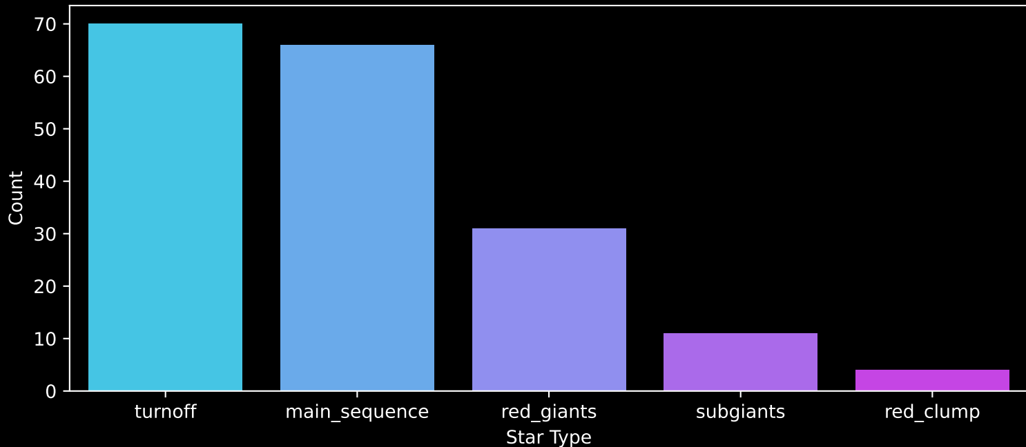
GALAH DR4 Field: [7156] Count plot of Star Type
